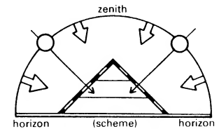
74 Constructional style suitable for northern regions (high proportion of diffuse light), side and overhead illumination
